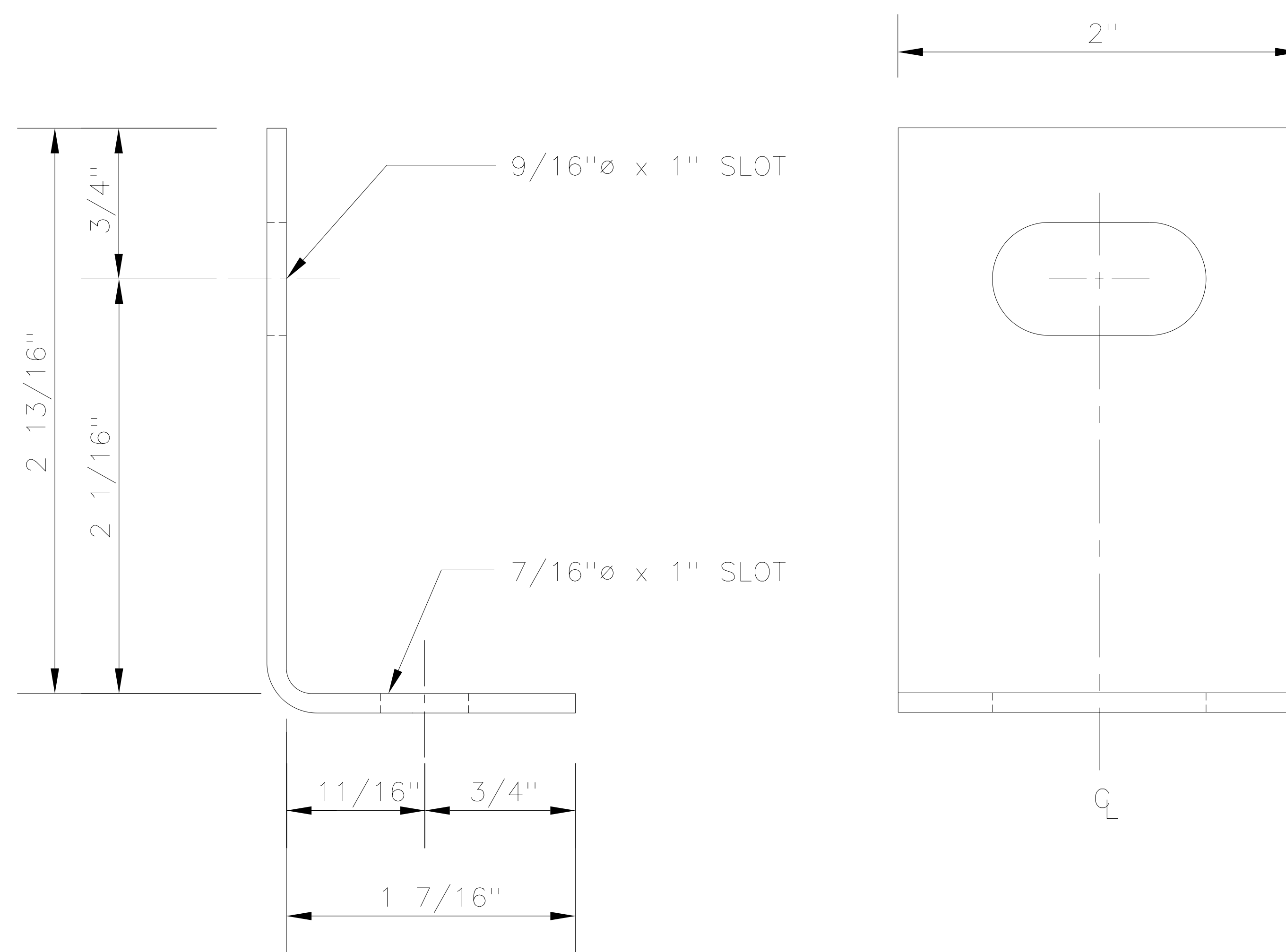
ROOF CAP SUPPORT ANGLE MK 353B12204 12 GA. x 4 1/4" x 2" FULL SCALE
