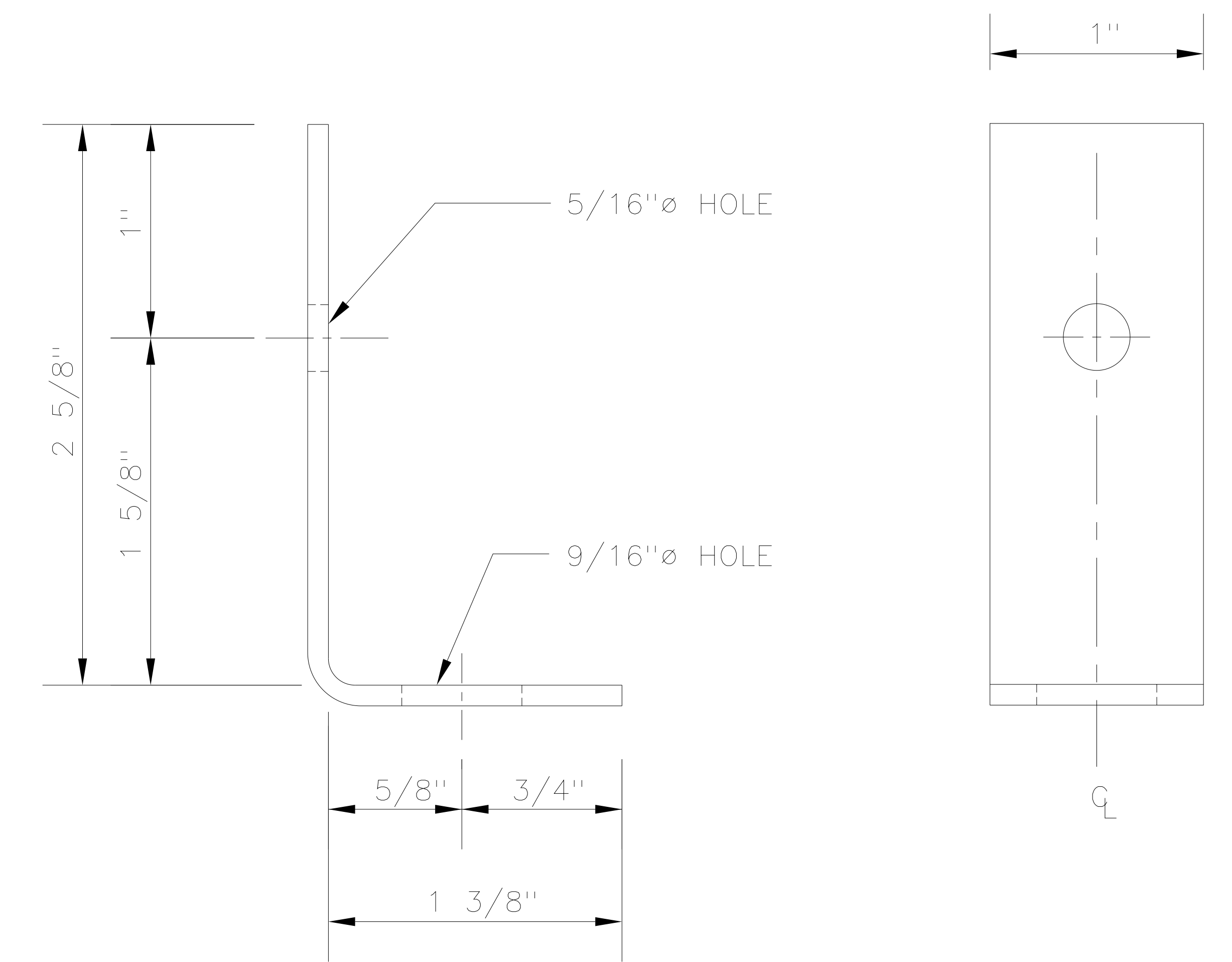
SCREEN SUPPORT ANGLE MK 353B12104 12 GA. x 4" x 1" FULL SCALE
