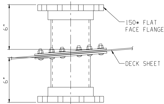
TYPICAL HILLSIDE DOUBLE FLANGED NOZZLE INSTALLATION
